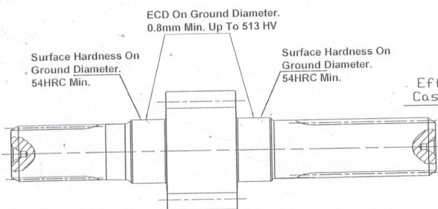
Figure i-1 Core Hardness Measured at this Location
