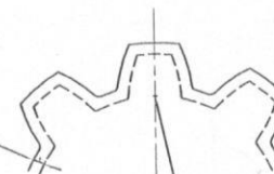
Figure i-1 Core Hardness Measured at this Location
